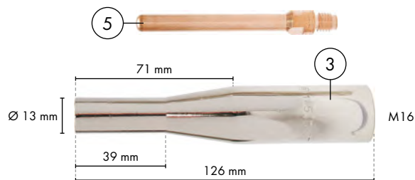
Gas nozzles and narrow gap gas nozzles for ABIMIG® A / A T
