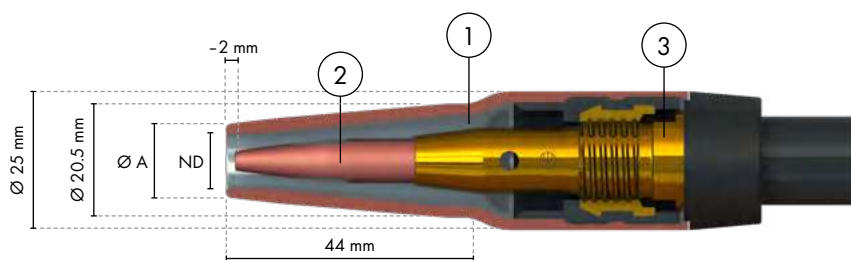
Narrow gap gas nozzle, tapered, for ABIMIG® A / A T 305 / 355 / 405
