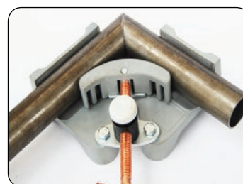
The rotateable spindle allows for holding work- pieces with different thicknesses.
